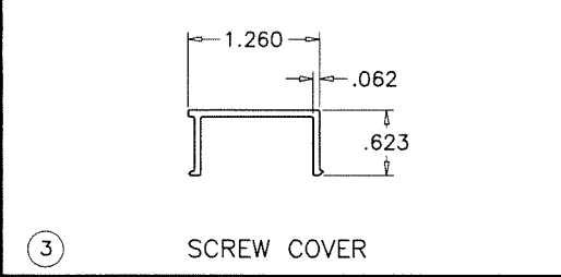
3 SCREW COVER
