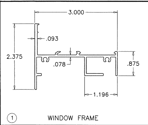
1 WINDOW FRAME
