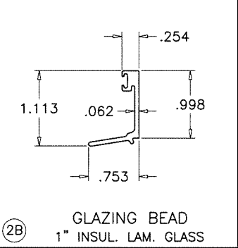
2B GLAZING BEAD 1" INSUL. LAM. GLASS
