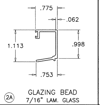
2A GLAZING BEAD 7/16" LAM. GLASS
