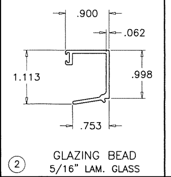
2 GLAZING BEAD 5/16" LAM. GLASS
